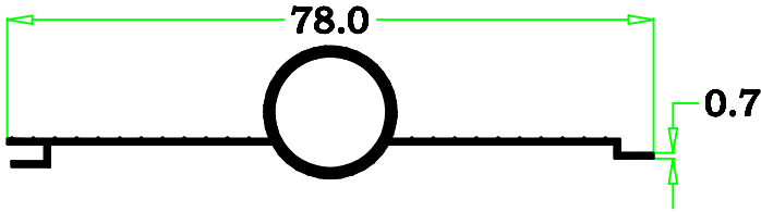
82-6 0.289 kg/m
