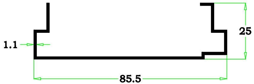
83-31 0.444 kg/m
