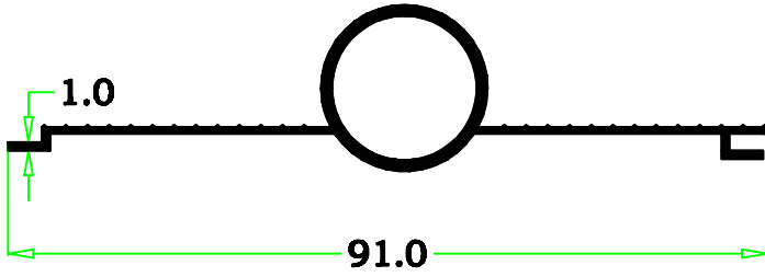
79-68 0.401 kg/m
