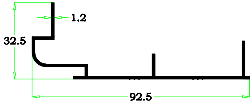
83-20 0.494 kg/m
