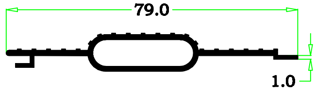
82-29 0.414 kg/m
