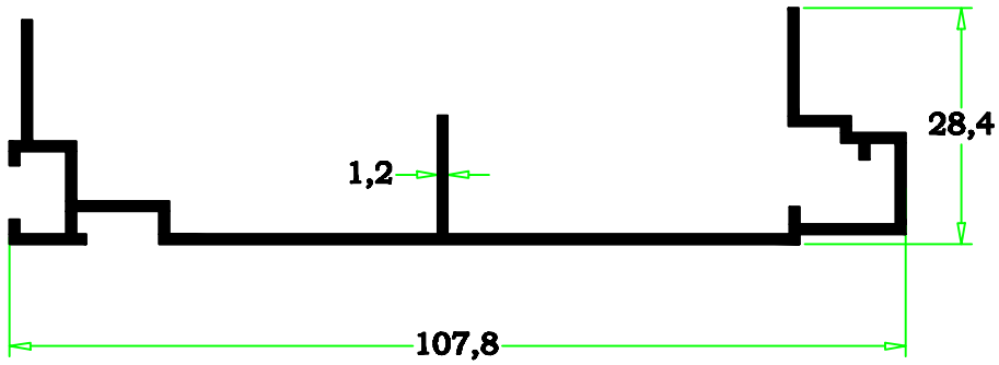
86-46 0.672 kg/m
