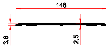
3078 1,095 kg/m
