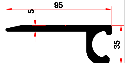
2990 1,897 kg/m
