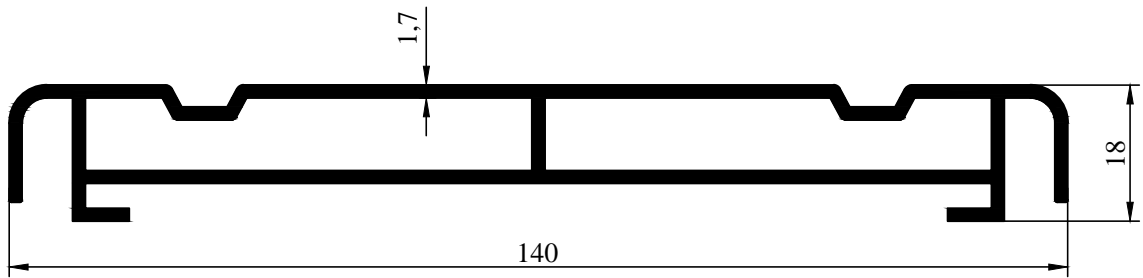
2981 1,586 kg/m
