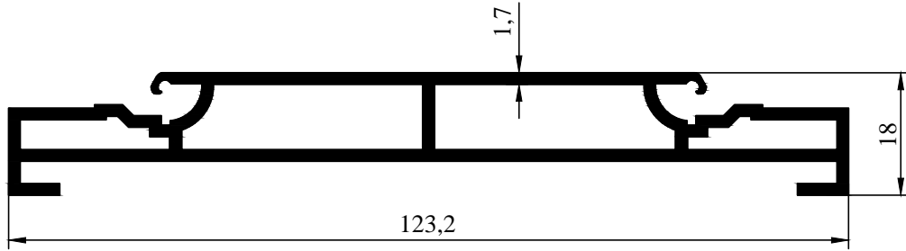
2982 1,475 kg/m
