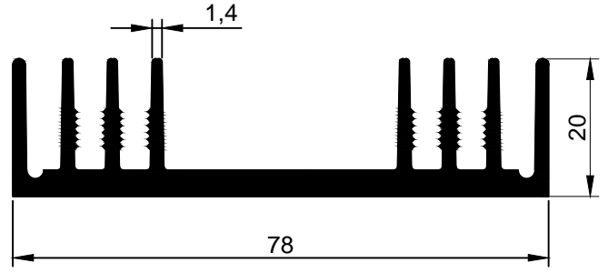
82-47 1,429 kg/m
