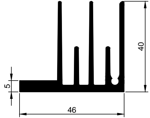
90-1 1,196 kg/m
