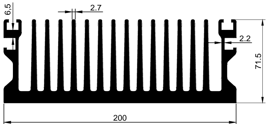
2972 16,053 kg/m
