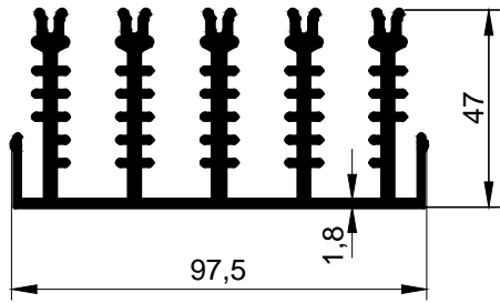
2970 2,987 kg/m
