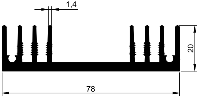
90-2 1,470 kg/m
