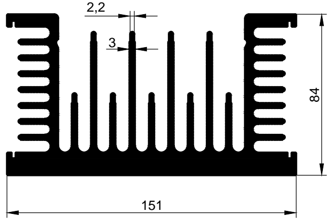
2971 11,837 kg/m
