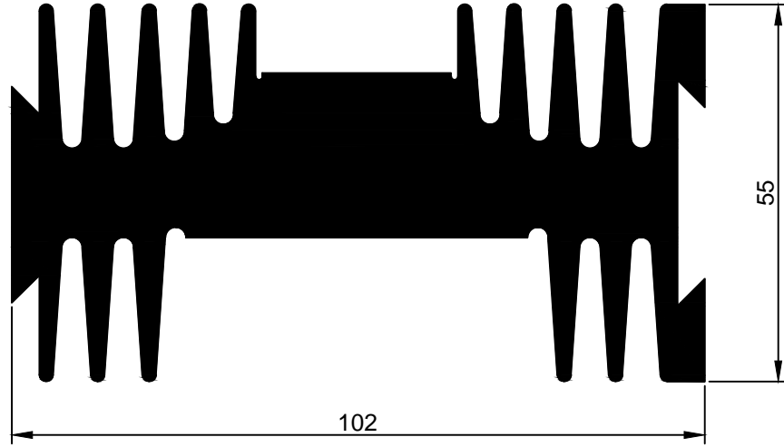
88-11 7,443 kg/m
