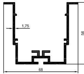
4336 1,046 kg/m
