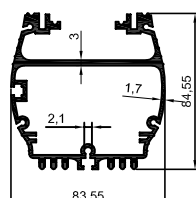
2950 2,935 kg/m
