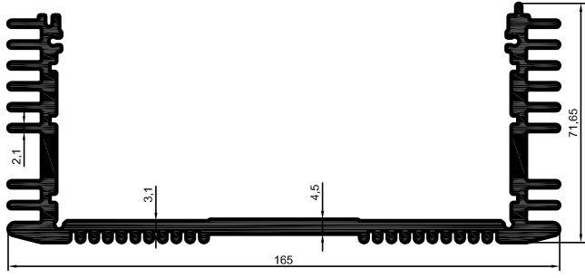
4136 4,537 kg/m
