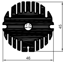
2008-79-B 3,368 kg/m
