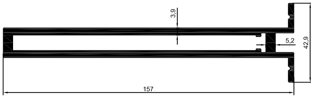
3893 3,699 kg/m
