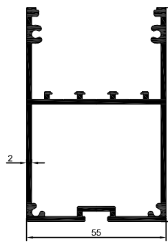
4177 1,776 kg/m
