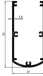
2008-05 1,071 kg/m
