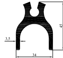
88-26 1,393 kg/m
