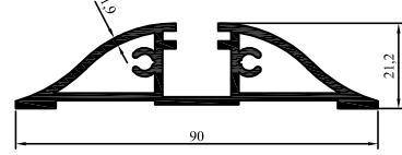
2005-13 1,222 kg/m
