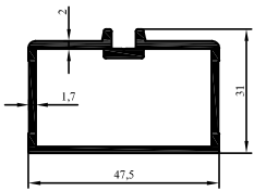
4276 0.759 kg/m
