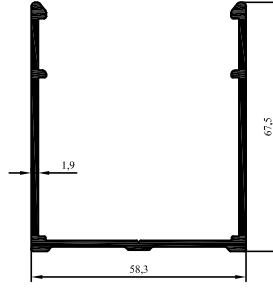
4272 1.053 kg/m
