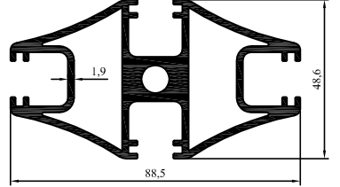
2005-106 2,560 kg/m
