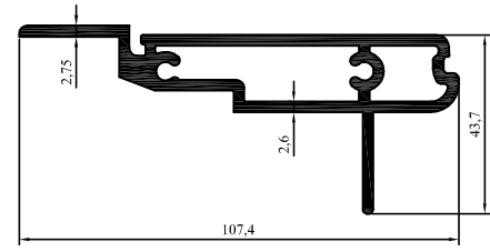
2000-11 1,955 kg/m
