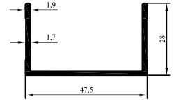
4275 0.459 kg/m
