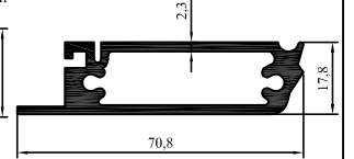
2000-9 1,179 kg/m
