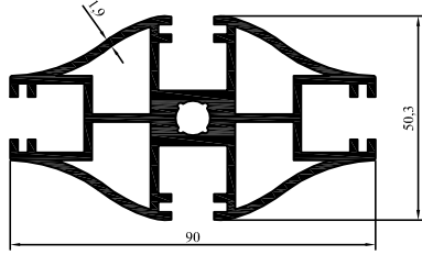
2005-14 2,610 kg/m
