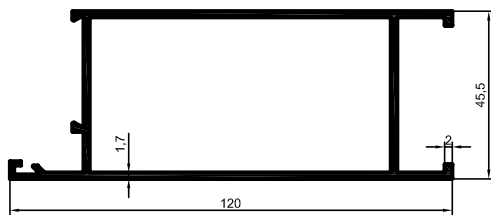
3482 1,474 kg/m
