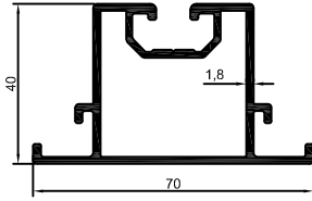
2006-60 1,166 kg/m
