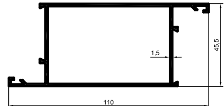
3484 1,182 kg/m
