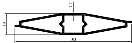
2003-60 1,102 kg/m
