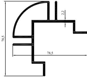
2000-78 1,453 kg/m
