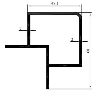
98-33 1,200 kg/m
