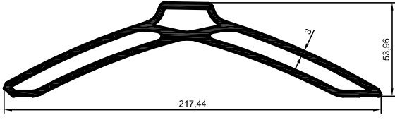
4662 4,219 kg/m
