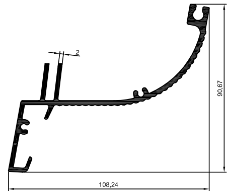
4661 1,665 kg/m
