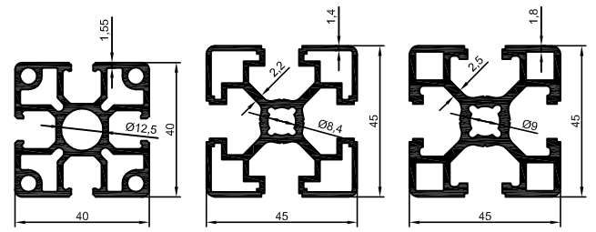
4378 1,414 kg/m 2006-78 1,362 kg/m 2006-90 1,672 kg/m
