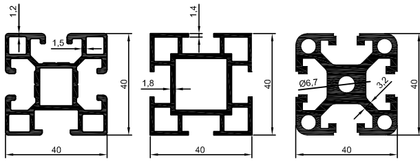
2006-66 1,150 kg/m 85-81 1,063 kg/m 3677 1,862 kg/m
