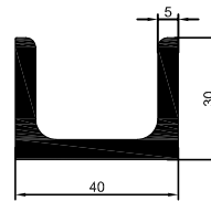
2011-43 1,242 kg/m
