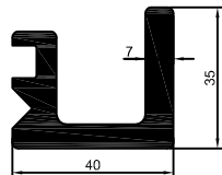
88-48 1,690 kg/m
